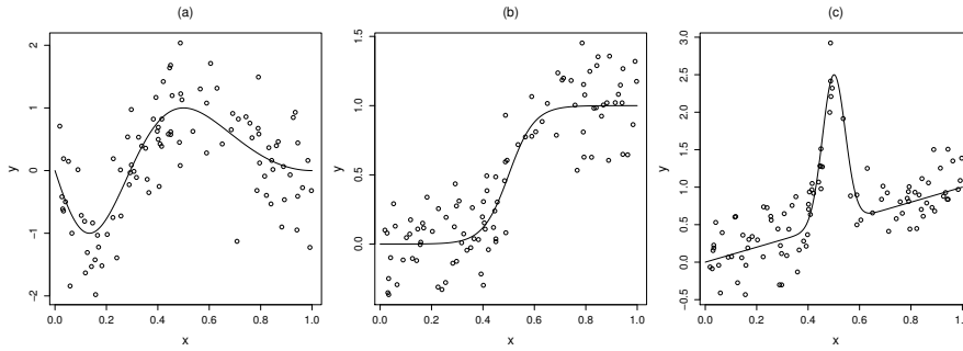
Fig. 1: Typical dataset for: (a) Cantoni and Ronchetti (2001) , (b) logistic and (c) “bump” test functions
