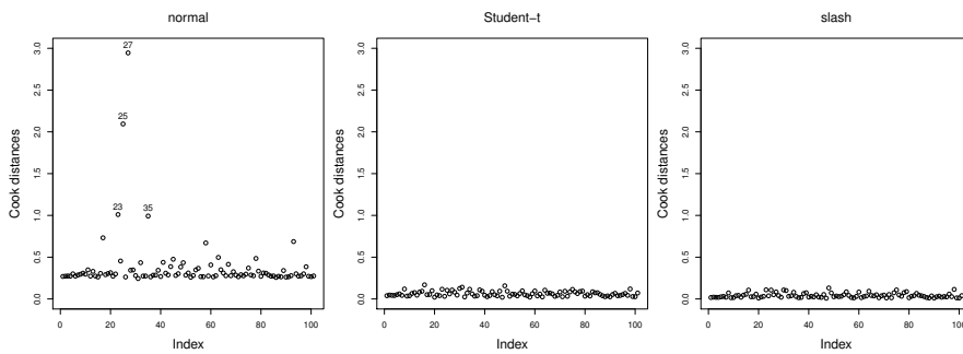
Fig. 10: Index plots of generalized Cook distances.
