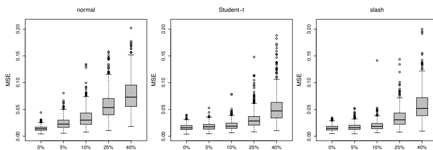
Fig. 6: Boxplots of MSE under several contamination levels ( \delta ) and variance inflation factor \gamma = 4 considering the three distributional assumptions for the “bump” test function.
