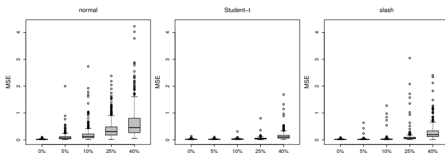
Fig. 3: Boxplots of MSE under several contamination levels ( \delta ) and variance inflation factor \gamma = 10 considering the three distributional assumptions for the Cantoni and Ronchetti (2001) test function.
