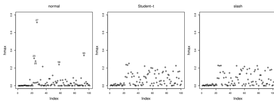
Fig. 11: Index plots of h_{\max} under scale perturbation on the penalized log-likelihood function.
