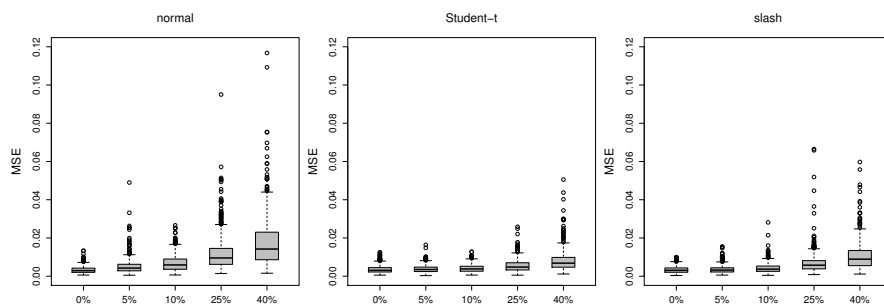
Fig. 4: Boxplots of MSE under several contamination levels ( \delta ) and variance inflation factor \gamma = 4 considering the three distributional assumptions for the logistic test function.
