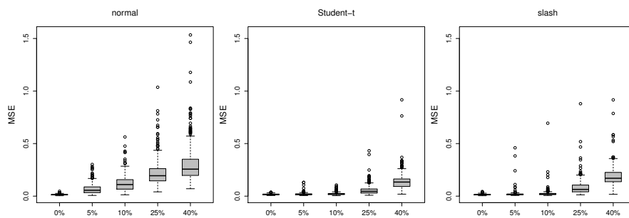
Fig. 7: Boxplots of MSE under several contamination levels ( \delta ) and variance inflation factor \gamma = 10 considering the three distributional assumptions for the “bump” test function.
