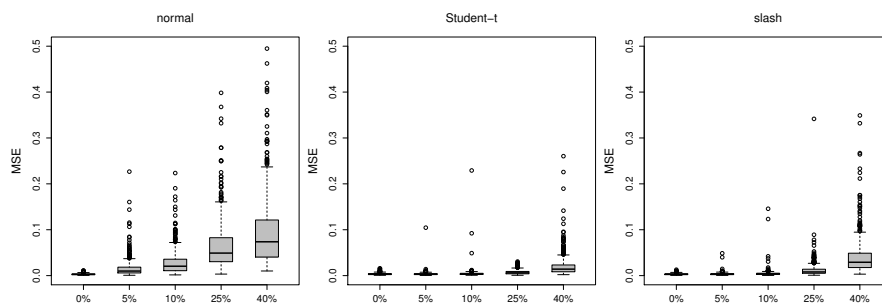
Fig. 5: Boxplots of MSE under several contamination levels ( \delta ) and variance inflation factor \gamma = 10 considering the three distributional assumptions for the logistic test function.
