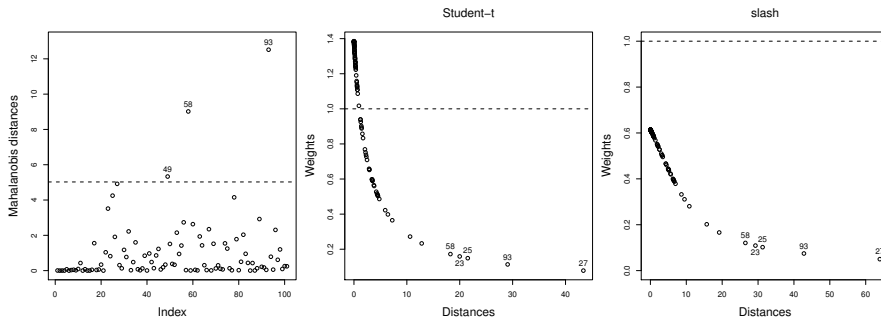
Fig. 9: Index plot of the Mahalanobis distances under normality and estimated weights versus distances for the Student- t and slash models.
