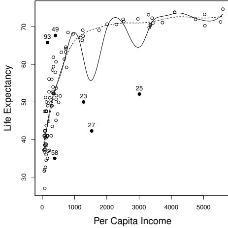
Fig. 8: Life expectancy data with fitted curve under three distributional assumptions: (—) normal, (- -) Student- t and ( \cdot\cdot\cdot ) slash models.
