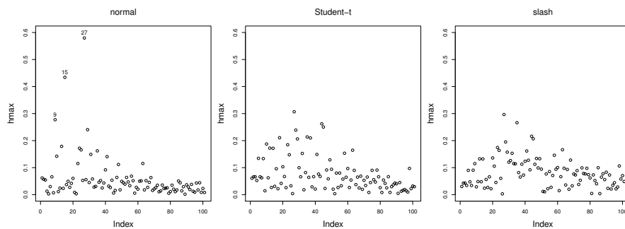
Fig. 13: Index plots of h_{\max} under scale perturbation on the smoothing parameter selection.
