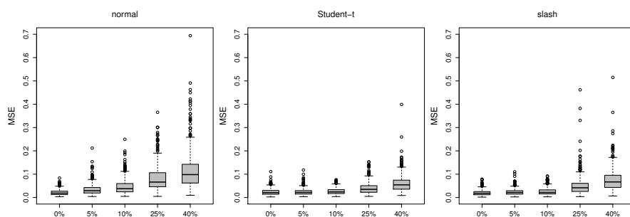
Fig. 2: Boxplots of MSE under several contamination levels ( \delta ) and variance inflation factor \gamma = 4 considering the three distributional assumptions for the Cantoni and Ronchetti (2001) test function.
