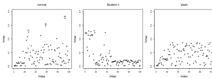
Fig. 12: Index plots of h_{\max} under response perturbation on the penalized log-likelihood function.
